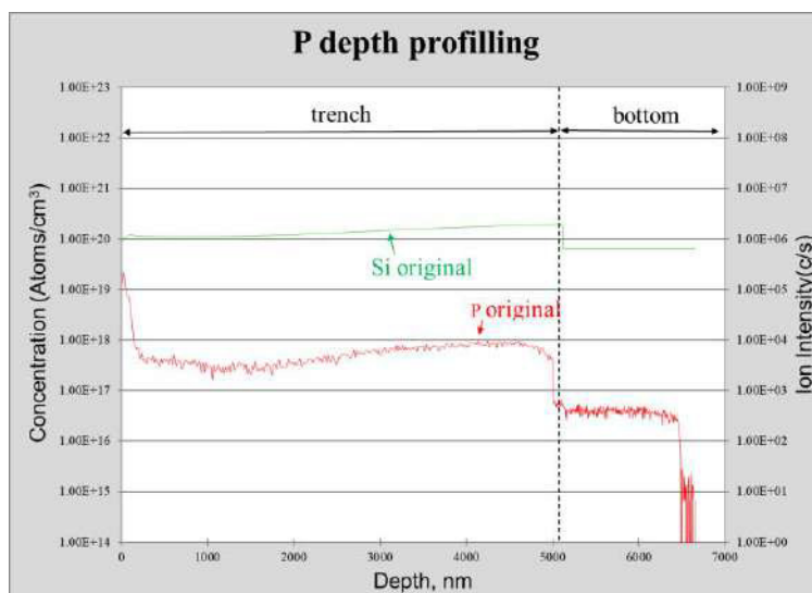
Figure 3. DSIMS depth profile in the original trench sample.
