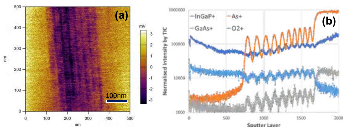
Figure 1. a) Conductance image showing the depth profile exhibiting contrast arising from the materials with different band gaps. The conductance is shown in a reverse falso color table, with dark meaning higher conductance and bright lower conductance. b) Depth profile of the same stack, exhibiting the composition modulation consistent with the nominal structure.
