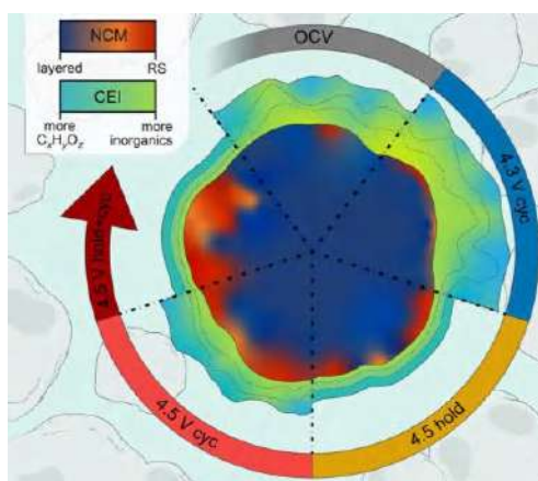
Figure 1: Post-mortem SIMS analysis of the CEI on NCM: schematic summary of the dependence of CEI composition on upper cutoff voltage and cycling protocol. [2]
