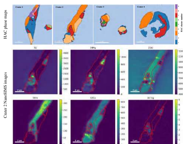
Figure 1. Top row: HAC-derived phase maps from four independent NanoSIMS measurements of the Al–Li alloy AA2395. Each color denotes a distinct compositional phase identified using the automated K-means/HAC workflow. Bottom two rows: Representative NanoSIMS total ion images from Crater 2 (selected isotopes shown), with red contours indicating HAC-derived phase boundaries corresponding to the phase map in the top row.
