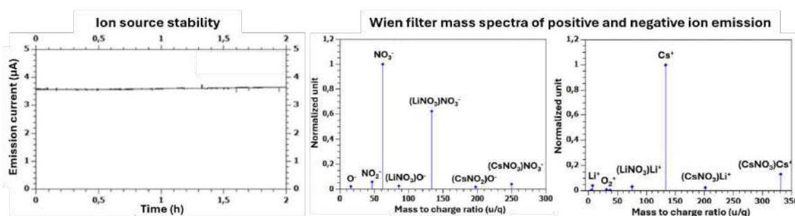
Figure 1: Ion source emission stability over two hours and wien filter mass spectra of positive and negative ion emission.
