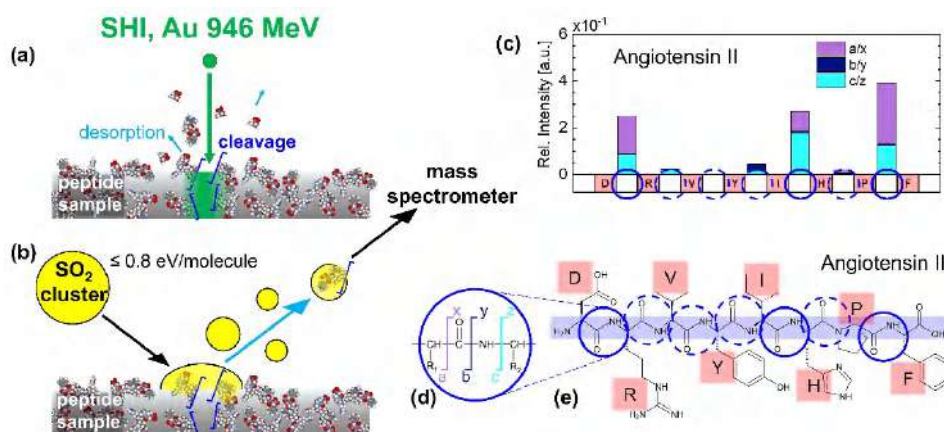
Fig. 1: (a) and (b) Fragmentation induced by SHI is analyzed by DINeC-MS. (c) to (e) The resulting distributions of fragments show high site-selectivity with respect to the cleavage site in the peptide.
