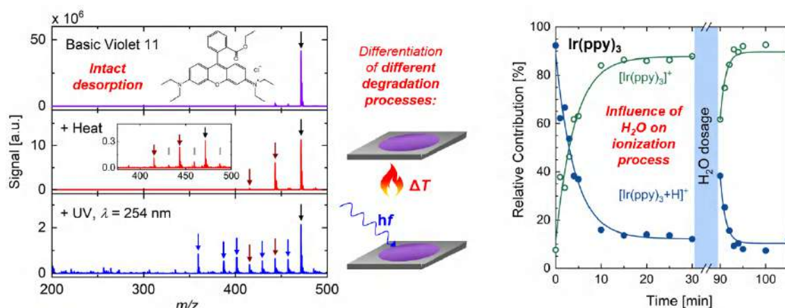
Fig. 1: Left: Intact desorption of basic violett and different fragmentation patterns induced by different stimuli. Right: Dependence of ionization process of OLED compound Ir(ppy) 3 on H 2 O supply.
