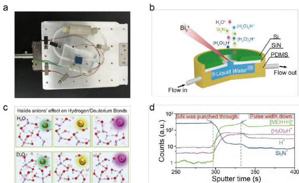
Figure 1. Schematic of in-situ liquid ToF-SIMS and characterized water clusters.
