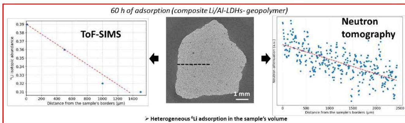
Fig. 1: Neutron tomography analysis of a composite after 60 h of adsorption
