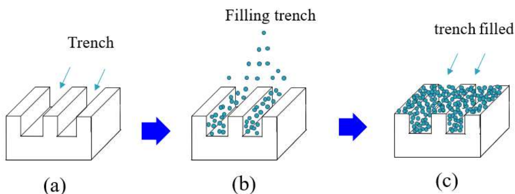
Figure 2. Schematic showing the trenches filled with \text{SiO}_2 .
