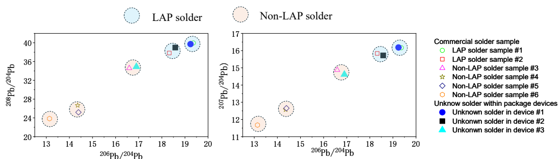
Figure 1. Lead isotope fingerprint reference map of solders used in microelectronic packages.
