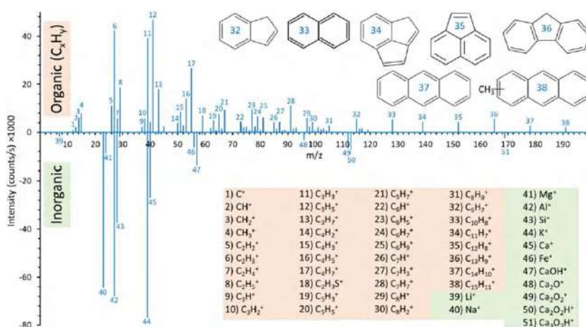
Figure 1. The TOF-SIMS mass spectrum at 450 °C in positive ion mode minus the mass spectrum at 25 °C. All the ion intensities were normalized against the summed total ion intensity prior to being subtracted in order to remove possible instrument effects.
