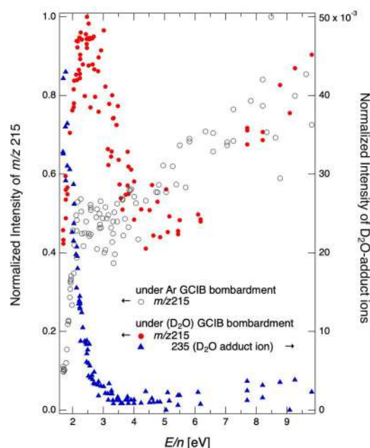
Figure 1 E/n dependence of the yields for the m/z 215 ions and the corresponding D 2 O adduct ions. The vertical axis is normalized with the maximum intensity for each species.
