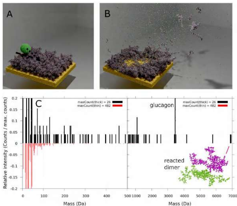
Figure 1. (A-B) 20 keV Ar 3000 -induced emission from a glucagon thick layer; (C) Comparison of the mass spectra computed from thick (black) and thin (red) layers.
