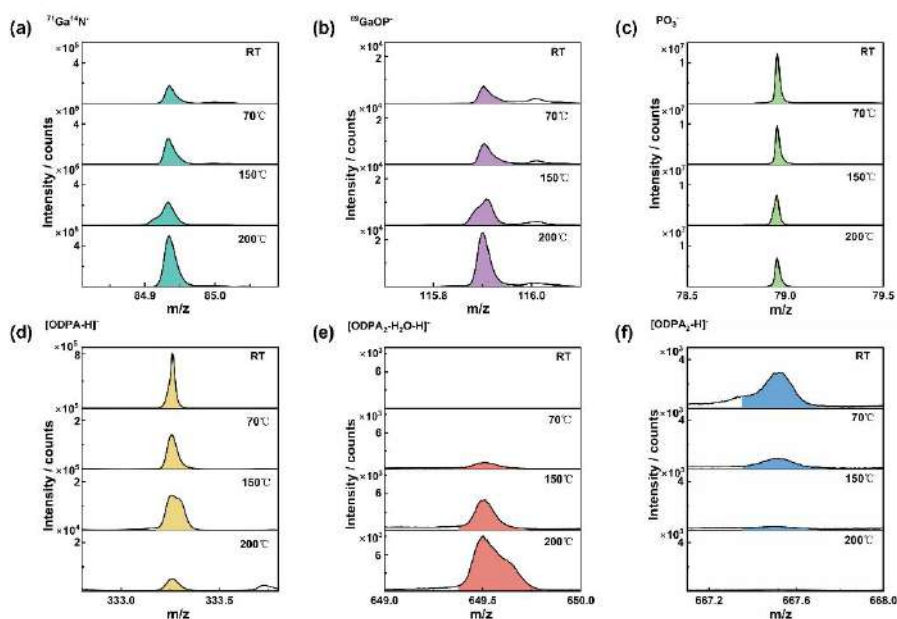
Figure 1. Temperature-dependent negative-ion ToF-SIMS spectra of ODPa-covered GaN after annealing from room temperature to 200 °C.
