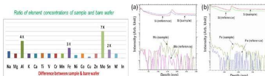
Fig.2. ICP-MS analysis was used for investigation and results showed abnormalities in aluminum (Al), iron (Fe), molybdenum (Mo), and tin (Sn) elements (left). D-SIMS quantitative analysis confirmed that the content of molybdenum and iron in the failed sample was higher than those in the normal sample (right).
