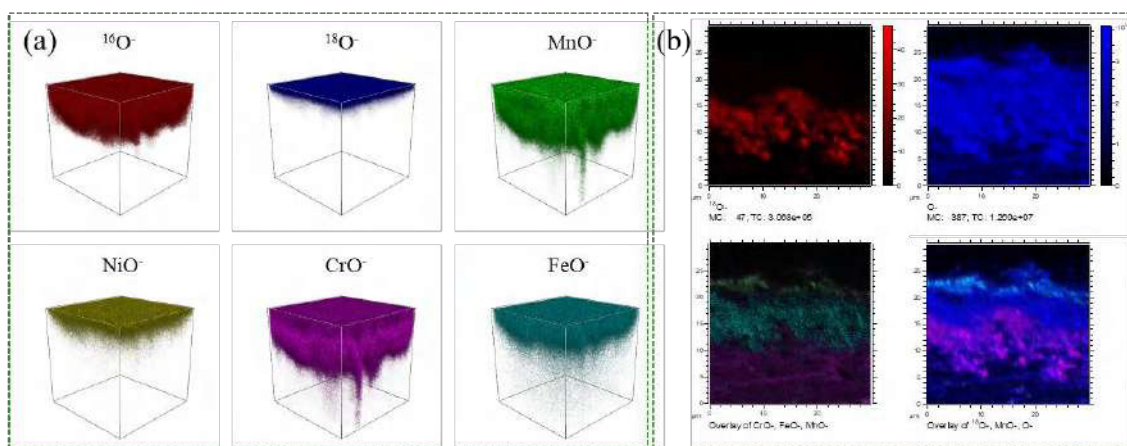
Fig. 1. Elemental distribution of oxide scales formed on stainless steel. (a) 3D isotope oxygen distribution in T91 steel after 5 h oxidation at 700 °C. The oxidation process consisted of two stages: from 0–1 h, the T91 steel was exposed to Ar-20% 16 O 2 mixed gas; from 1–5 h, it was exposed to Ar-18% 16 O 2 -2% 18 O 2 . (b) Overlay isotope oxygen distribution in 310S steel after 20 h oxidation at 1100 °C. The oxidation process also consisted of two stages: from 0–5 h, the 310S steel was exposed to Ar-18% 16 O 2 -2% 18 O 2 mixed gas; from 5–20 h, it was exposed to Ar-20% 16 O 2 . Red, blue, green, magenta, and cyan represent 18 O - , 16 O - , MnO - , FeO - , and CrO - ions, respectively.
