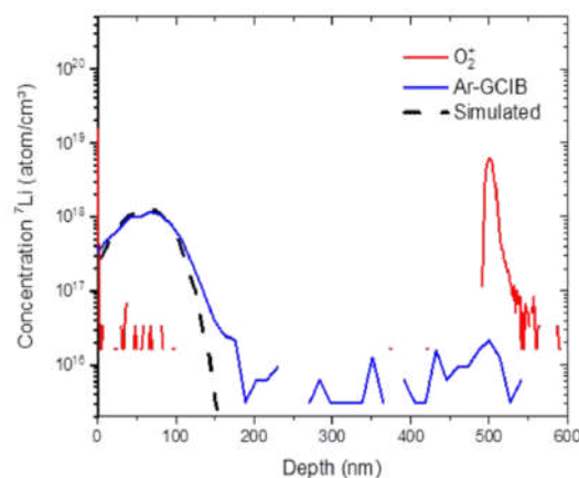
Figure : Comparison of ToF-SIMS depth profiles of Lithium in thermally grown silicon oxide using different sputter ion species
