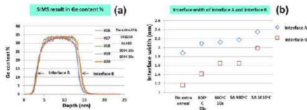
Figure 2. Figure 2 (a) shows a SIMS profile on same sample with APT. 1 (b) shows an interface diffusion defined by profile.
