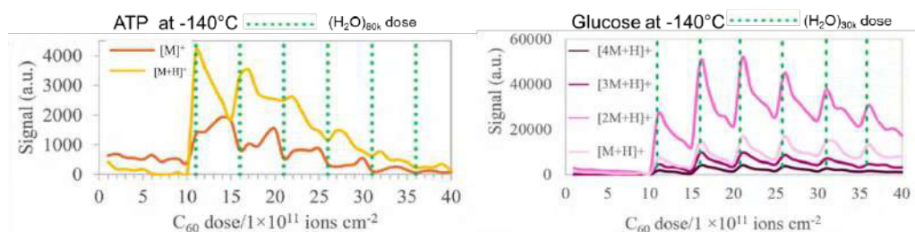
Figure 1 - Illustrates the enhancement of water-GCIB dosing on the C_{60} -SIMS analysis of a molecular surface.
