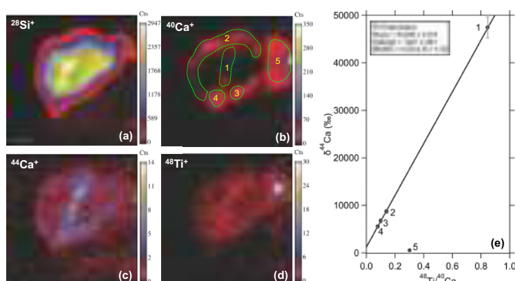
Figure 1. Panels (a) to (d) show the ^{28}\text{Si} , ^{40}\text{Ca} , ^{44}\text{Ca} , and ^{48}\text{Ti} ion images of an X grain. The white scale bar in panel (a) denotes 500 nm. In panel (b), different regions of interest (ROIs) were defined for reducing the Ca-Ti isotope data in panel (e). Errors are all 1\sigma . The data for ROI #5 was excluded from the linear fit because of its significant deviation (Adapted from [5]).
