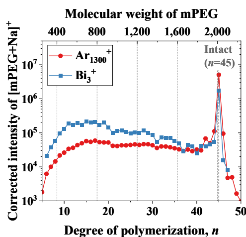
Figure 1. Comparison of molecular weight distributions of singly-charged mPEG ions by Ar gas cluster and Bi cluster irradiation.
