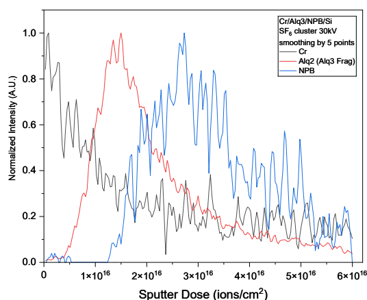
Figure 1. Depth profile of the organic-inorganic multilayer device using SF 6 gas cluster ion beam at 30 kV.
