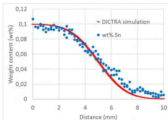
Figure 1. Concentration gradient in a diffusion couple.
