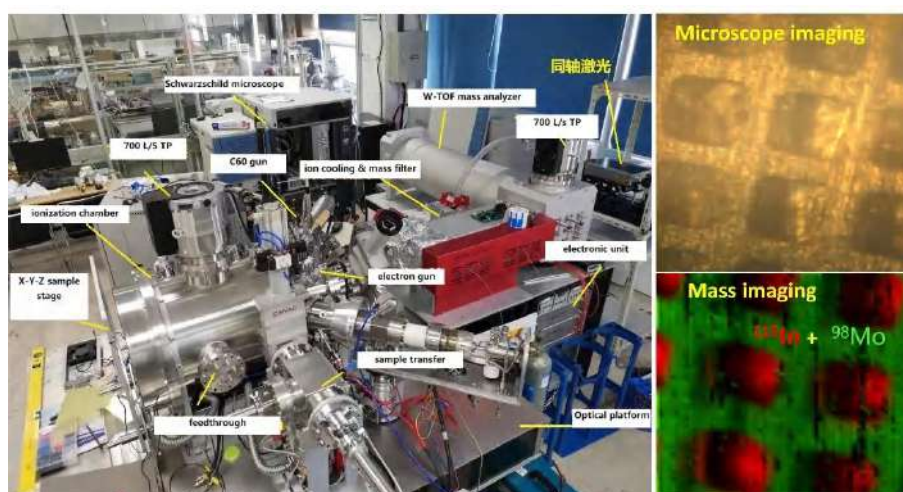
Figure 1. (a) Instrument overview of the correlated microscope/SIMS imaging mass spectrometry. (b) Microscope imaging of the 200-mesh molybdenum mesh and Indium foil surface. (c) Mass imaging of the 200-mesh molybdenum mesh (green) and Indium foil surface (red).
