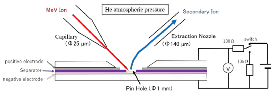
Fig.1 Schematic diagram of a holder specifically for operando MeV-SIMS measurement.
