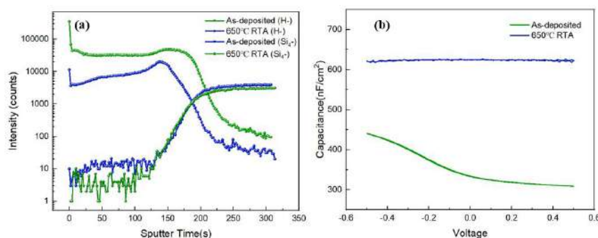
Figure 1. (a) Comparative TOF-SIMS depth profiles of AIBN films. Using \text{Si}4^- as an interface marker, a pronounced relative decrease in bulk \text{H}^- intensity is observed after 650 °C RTA. (b) Corresponding C-V curves demonstrating the transition from a trap-induced distortion to a flat, intrinsic dielectric plateau with enhanced capacitance.
