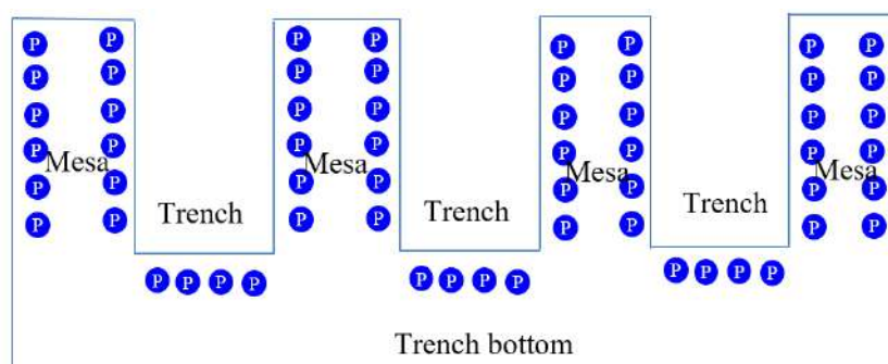
Figure 1. Schematic structure of the SiC trench sample. P dopants are in the mesa walls and trench bottoms.
