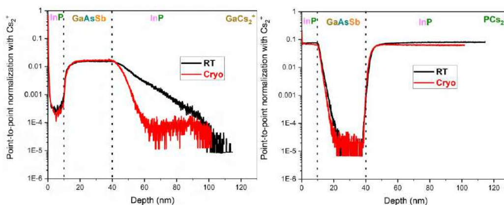
Figure 1. Overlay of positive polarity ToF-SIMS depth profiles acquired at room temperature (black) and under cryogenic conditions (red) respectively for \text{GaCs}_2^+ (left) and \text{PCs}_2^+ (right) [3].
