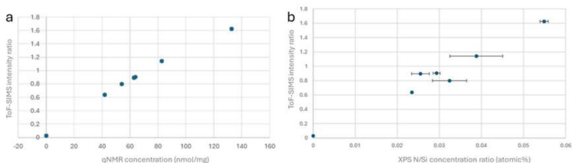
Figure 1 Correlation between ToF-SIMS intensity ratios (peaks representing amine/silica) and (a) amine concentration determined by qNMR, and (b) XPS atomic concentration ratio (N/Si).
