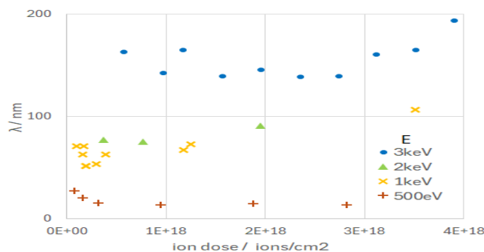
Fig.2 Examples of \lambda variation with ion dose at \theta=45deg .
