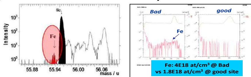
Fig.1. TOF-SIMS survey found Fe contamination on the failed sample (left). D-SIMS detected Fe contamination on the bad sample (right).
