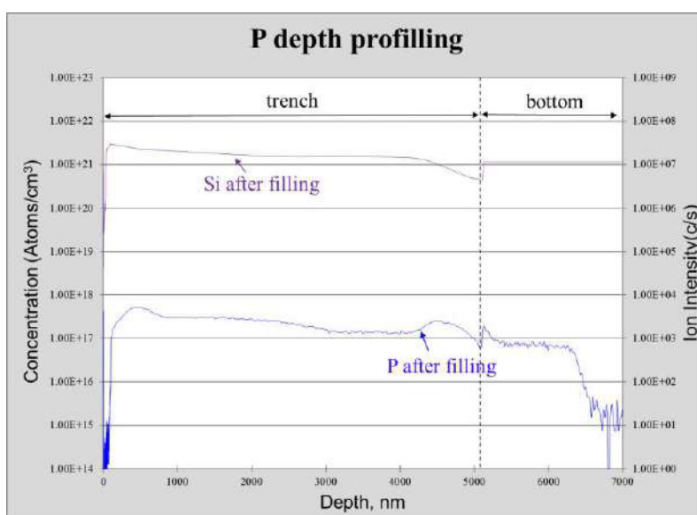
Figure 4. DSIMS depth profile in the SiO 2 -filled sample.
