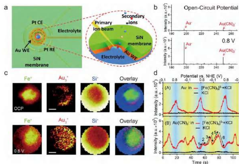
Figure 1. Concept of ToF-SIEMS probing the EEl)s through the pore confined configuration.
