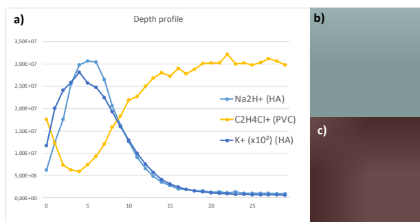
Figure 1. a) Depth profiles for secondary ions species associated to HA and PVC. Secondary ions intensity map for b) Na2H^+ and c) C2H4Cl^+ mass spec peaks.
