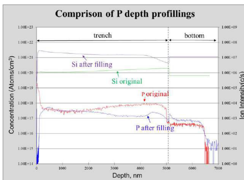
Figure 5. Comprison of DSIMS depth profiles in the original and SiO 2 -filled samples.
