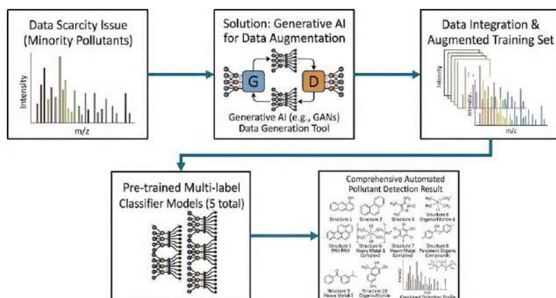
Figure 1. An integrated framework for minority pollutant detection via GAN-driven mass spectrometry data augmentation and multi-label classification.
