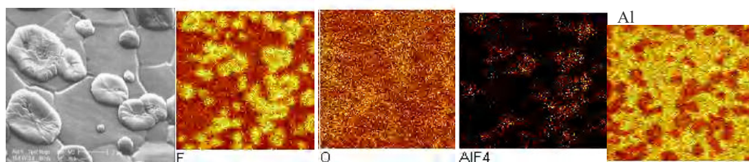
Fig.1. SEM photo of the defects and the detection of [\text{AlF}_4]^- ions by TOF-SIMS ion mapping confirms the presence of [\text{AlF}_6]^{3-} .
