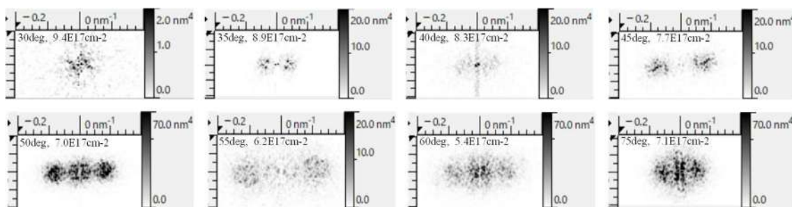
Figure 1. Typical variation of 2DPSD with \theta at low dose levels ( E=2keV ) \theta and ion dose are shown in each 2DPSD.
