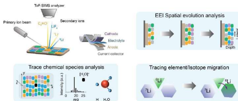
Figure 1. Schematic illustration of characteristic applications of ToF-SIMS in battery interface characterization.
