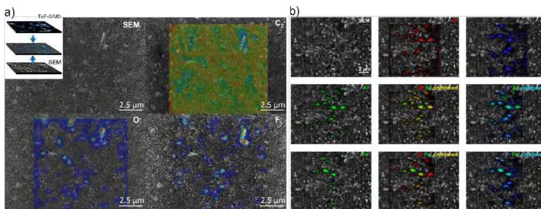
Figure 1. a) SIMS negative mode images on SEM image of a complex carbon-based matrix consisting of functionalized graphene flakes and carbon black (inset illustrates the idea of correlative analysis) and b) metal impurities and their overlapping in position with F - and O - fragments in the same matrices.
