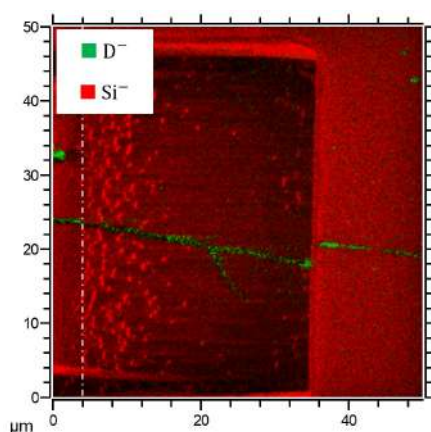
Figure 1. ToF-SIMS image overlay of Deuterium (green) and Silicon (red) in negative ion detection mode of a FIB crater on a crack that was stored in a container with heavy water for 14 days; Instrument: M6 Plus
