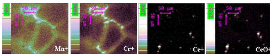
Figure 1. Intensity maps for Mn + , Cr + , Ce + and CeO + mass peaks.
