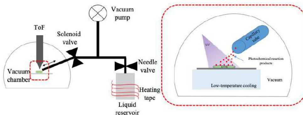
Figure 1. Schematic illustration of a vacuum-compatible system integrating vapor-phase deposition, in situ reaction, and ToF-SIMS imaging.
