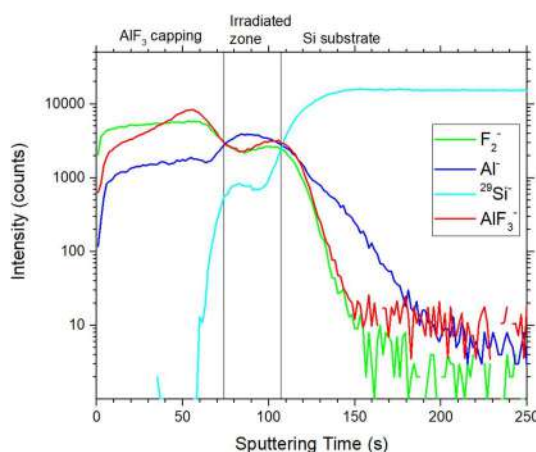
Figure 1. TOF-SIMS depth profiling of a sample consisting of a Si substrate, an \text{AlF}_3 layer irradiated with low-energy electrons and a non-irradiated \text{AlF}_3 layer for capping.
