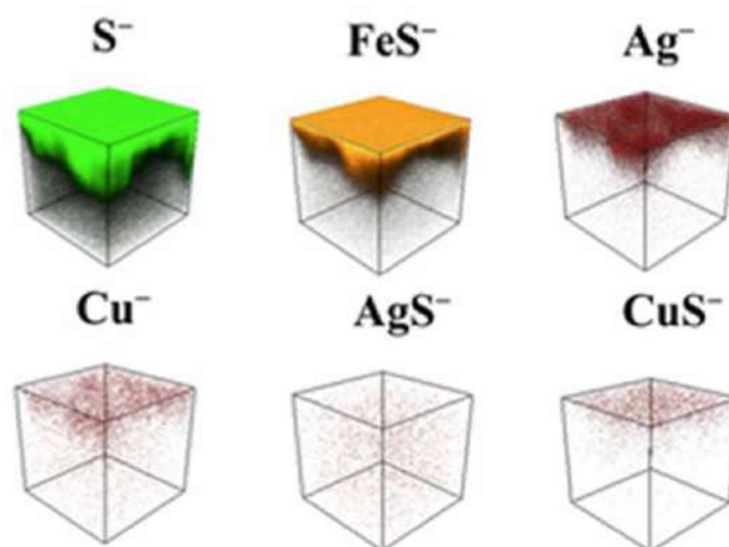
Figure 1. 3D ToF-SIMS images of the produces species after treatment with Cu-Ag BNP hydrosol
