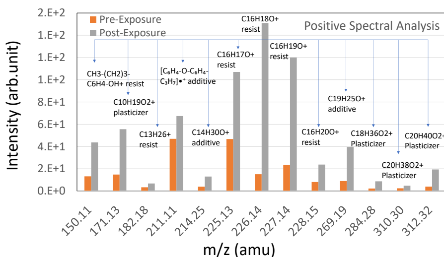
Figure 1. Some of the signature mass peaks assigned from the photoresist for post exposure versus pre exposure
