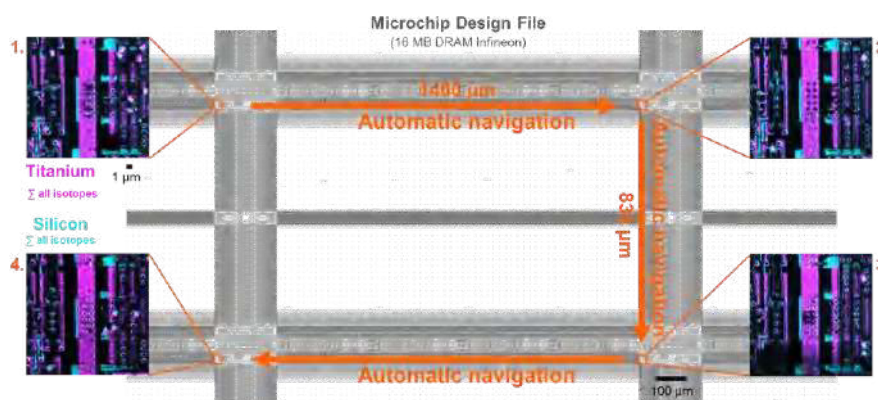
Fig. 1. Automatic nm-precise sample navigation workflow with subsequent high-resolution SIMS imaging of a 16 MB DRAM Infineon microchip. Recorded SIMS maps of Titanium and Silicon are shown in magenta and cyan, respectively.
