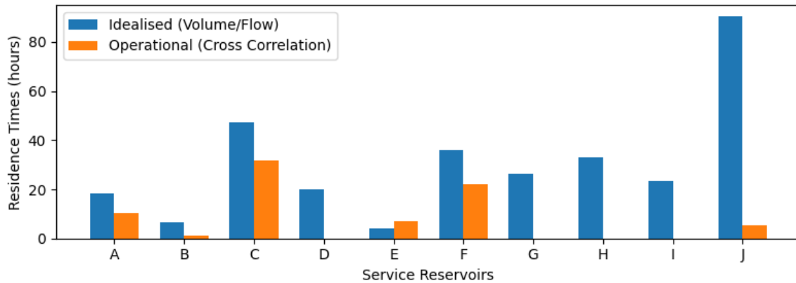
Figure 77 Idealised and operational residence times for ten service reservoirs.
