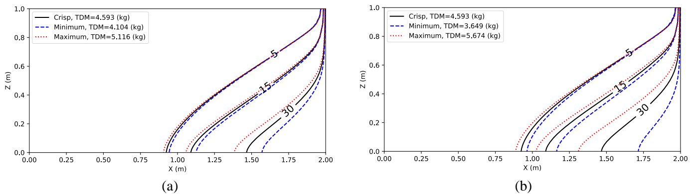
Figure 2. Uncertainty analysis results for Henry’s problem, a) 5% uncertainty and b) 10% uncertainty
