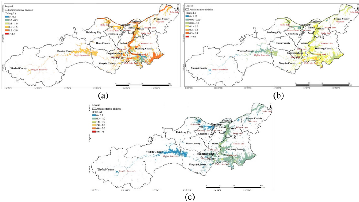
Figure 1 Water quality parameters inversion result based on remote sensing ((a) is TN, (b) is TP, (c) is Chla)
