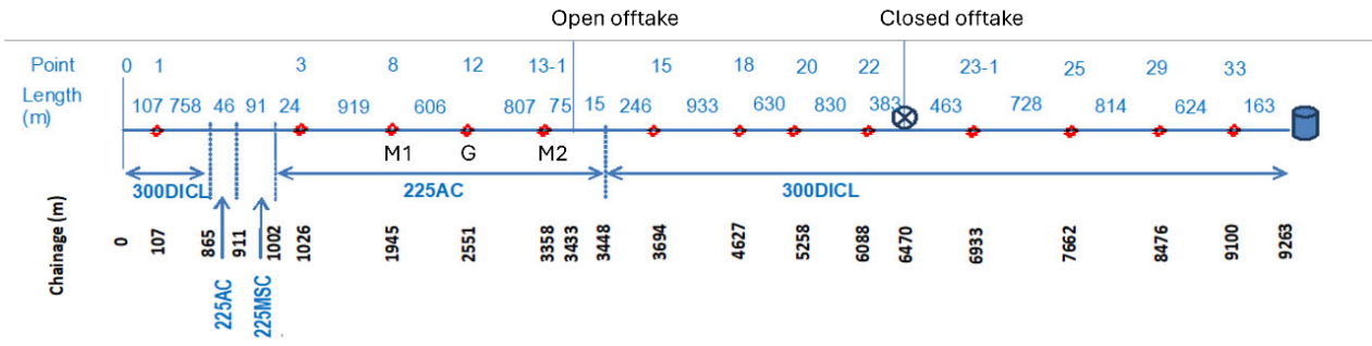
Figure 1. Layout of the field pipe system.
