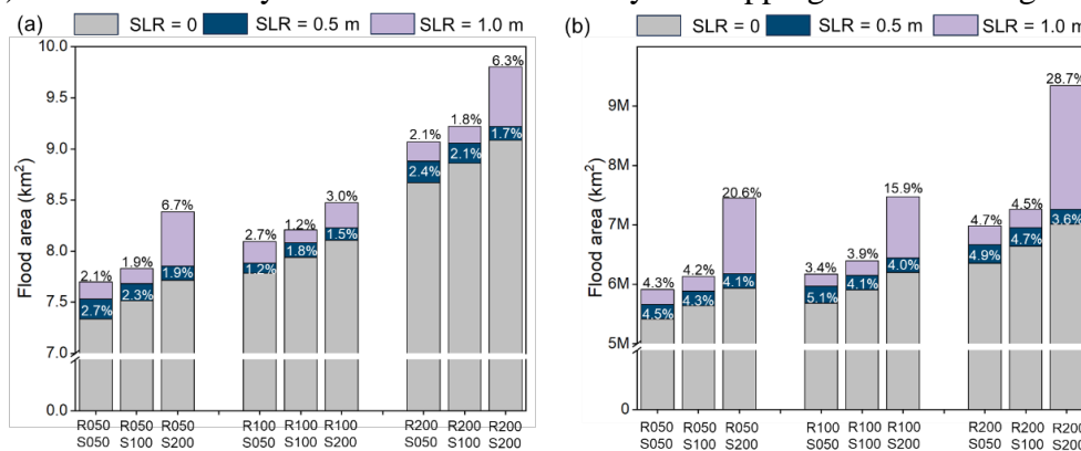
Figure 1 (a) Areas and (b) Volume affected by flooding and inundation with SLR, progressive storm surge heights and rainfall (cumulative). Note: The height of the bar chart is the relative increase.
