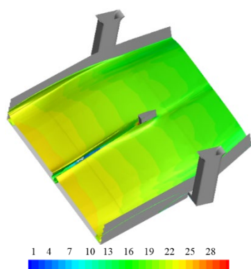
Figure 3 Water-surface profile (case 2) colored by velocity magnitude
