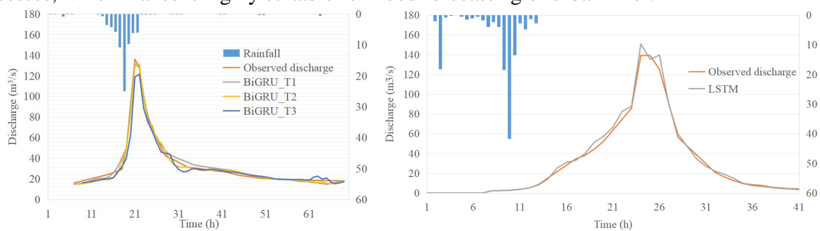
Figure 37 Illustration of flood forecasting results
