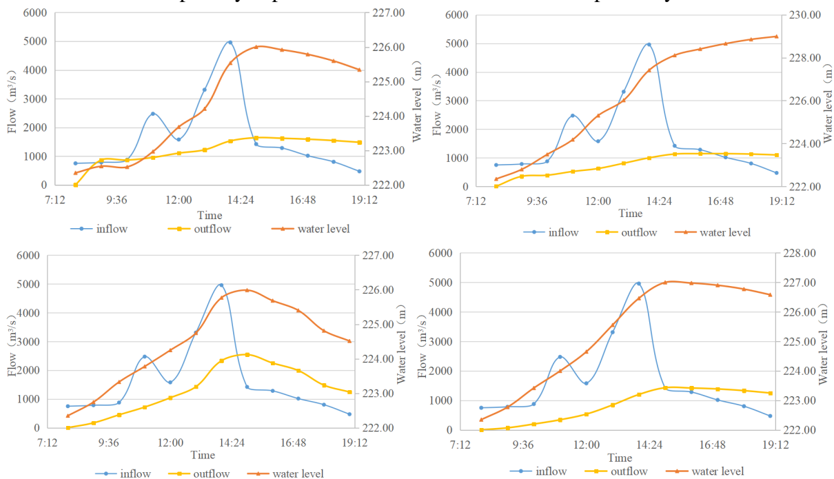
Figure 30 Calculation result of spillway expansion scheme of Xinfa Reservoir (a.excavation depth of the spillway is 6.1m; b.excavation depth of the spillway is 3.0m; c.the expansion widths of the spillway is 140m; d. the expansion widths of the spillway is 40m )
