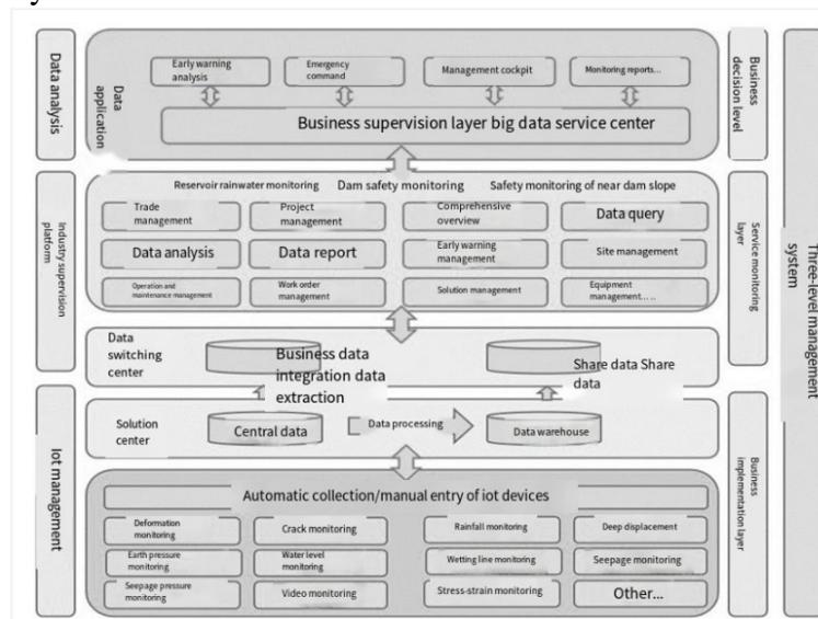
Figure 57 Multi-sensor-based rainwater monitoring and dam safety monitoring system architecture
