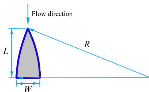
Figure 1 Splitter formed by two arcs
