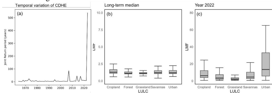
Figure 1. The temporal variation of CDHW in Sichuan Province.
