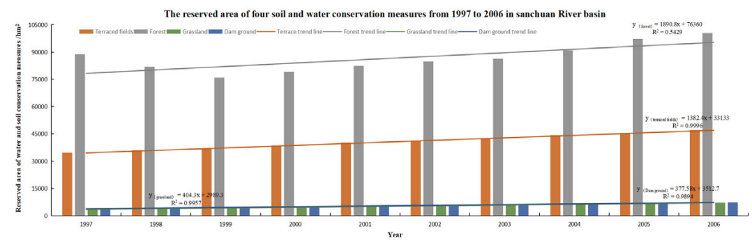
Figure 1 Reserved area of water and soil conservation measures from 1997-2006 in Sanchuan River basin
