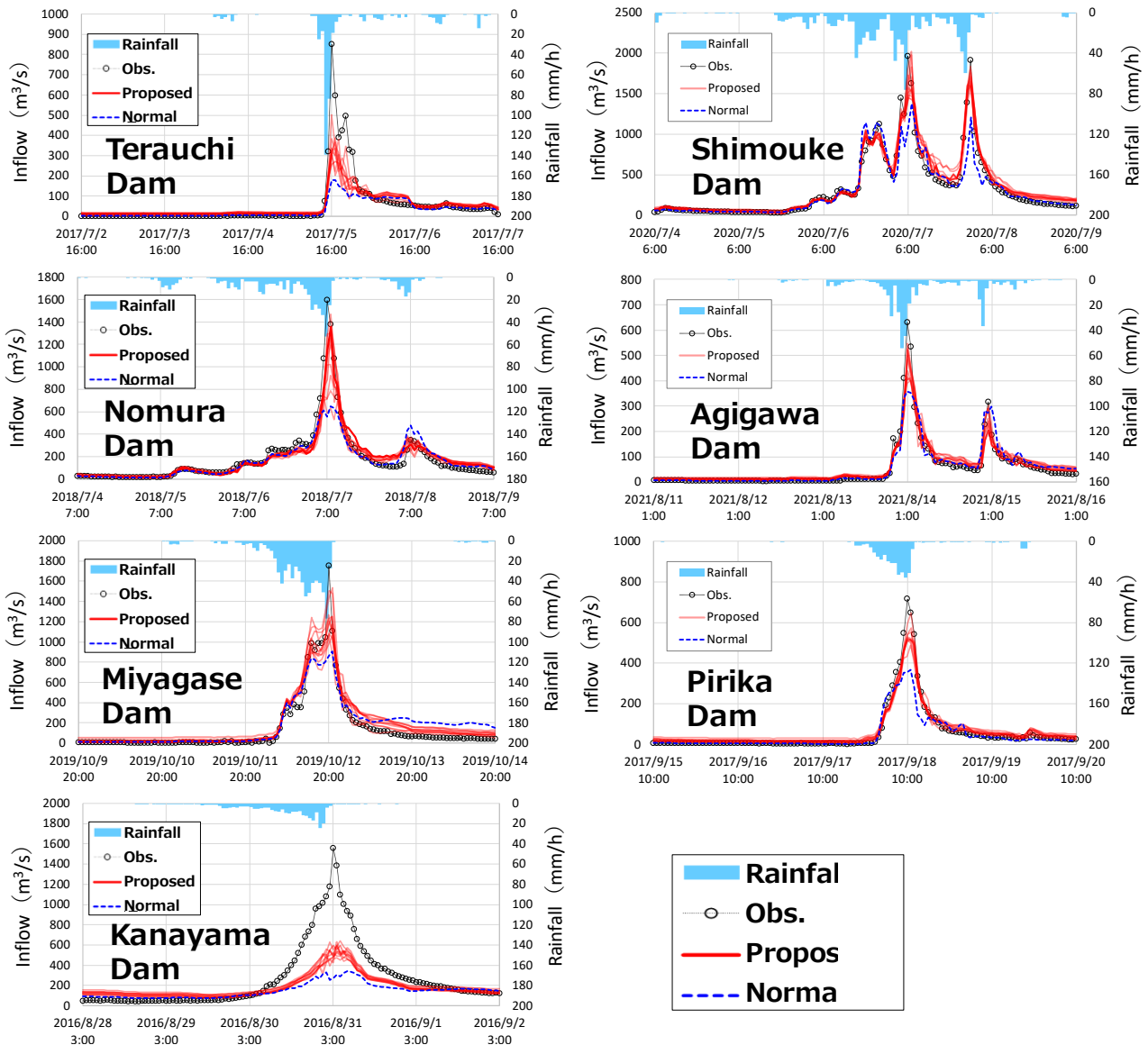
Figure 32 Results of test calculations for the largest floods in each dam
