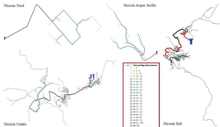
Figure 1. Domain analysis of the four subnetworks of the Nicosia WDN.
