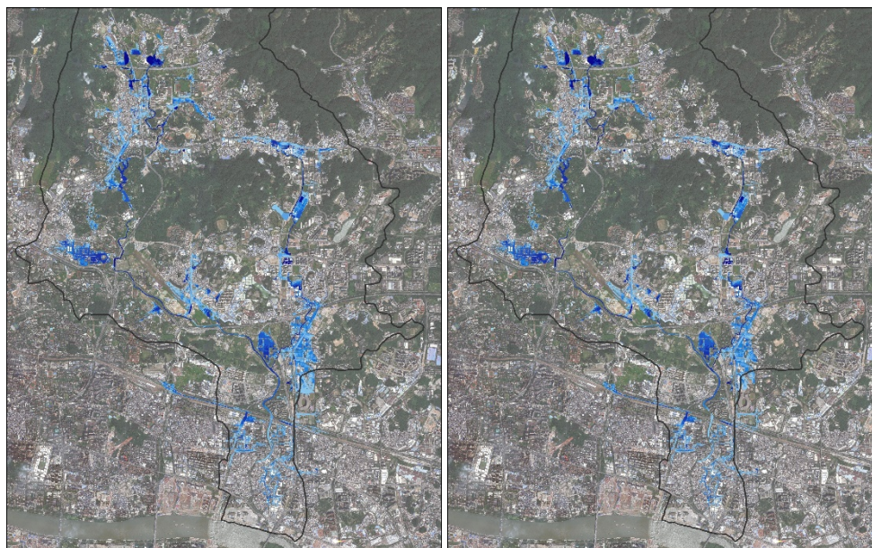
Figure 1. The simulated inundation water depth predicted using the CNN model (left) and the coupled model (right) under 50a test rainstorm scenarios ( t=2.0h ).
