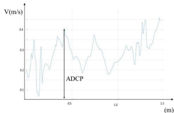
Figure 2 Comparison of velocity determined by image analysis with ADCP measure
