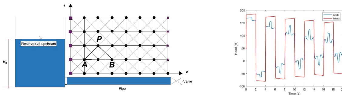
Figure 1 Schematic of an RPV system with discrete grids and Transient wave behaviour in an intact and leaking pipes.
