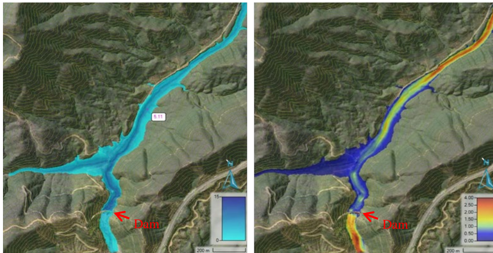
Figure 15 Maximum water depths (left, in m) and velocities computed with HEC-RAS (right, in m. s -1 )
