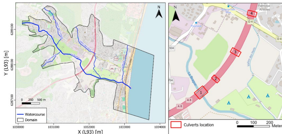
Figure 1 (a) The study area with the Brague river and its tributaries, (b) culvert location below the highway.
