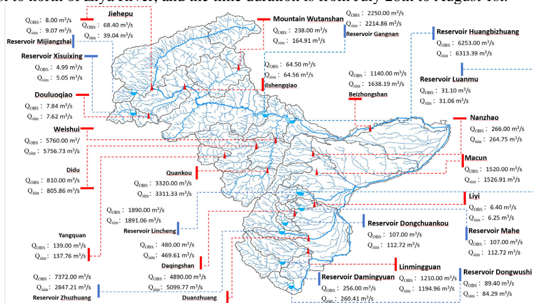
Fig1. The modelling results of “23.7” catastrophic flood in Ziya River Basin
