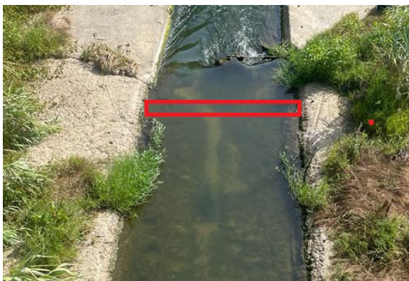
Figure 2 Comparison of velocity determined by image analysis with ADCP measure
