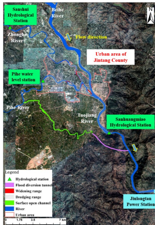
Figure 2. Layout of flood control engineering measures.
