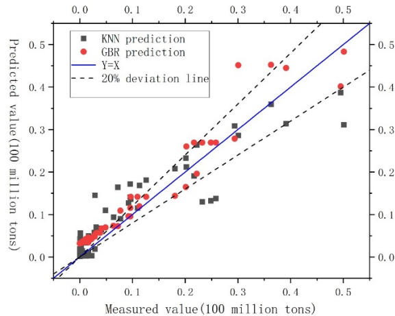
Figure 6 Correlation analysis between predicted and true values
