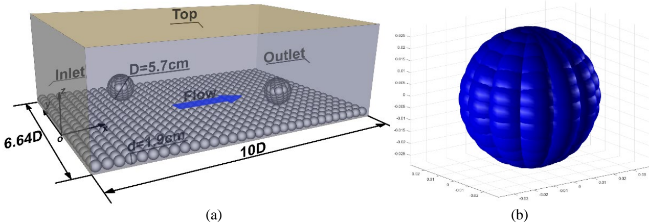
Figure 1 (a) Computational domain and (b) represented boulder.
