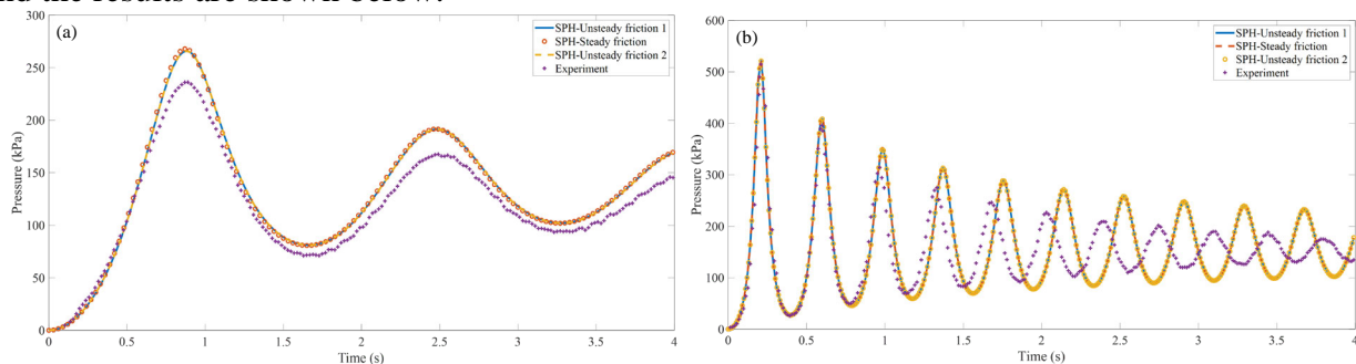
Figure 1. Comparison between numerical results of SPH with steady friction, SPH with unsteady friction and experiment, air pocket governing equations are polytropic process equation used in SPH-Unsteady friction 1 and Martin’s model [2] used in SPH-Unsteady friction 2, respectively: (a) Zhou et al. [3], (b) Zhou et al. [4]
