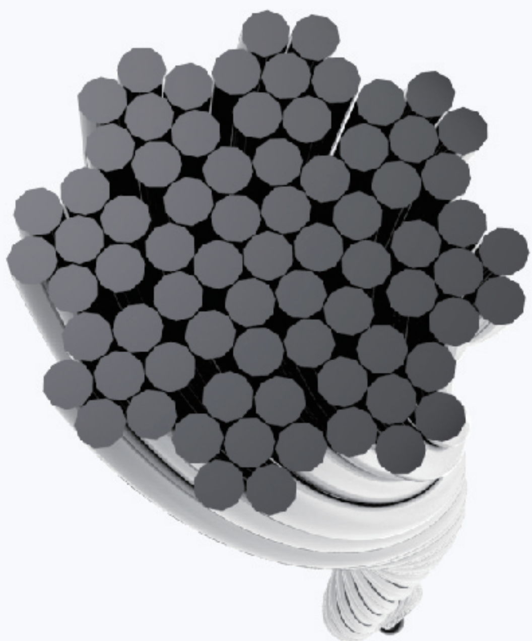
缆索 1 \times 19 + 8 (1 \times 7) = 75
