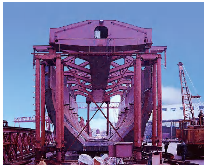
造桥机制作 Fabrication of bridge building machine
