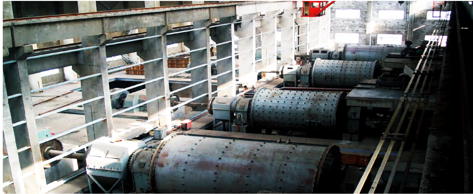
山西铝厂选矿工程 Shanxi Aluminum plant beneficiation project
