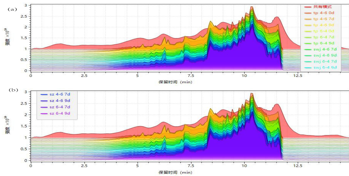
Figure 1 UPLC-MS / MS establishes the fingerprint of secondary metabolites in different culture systems
